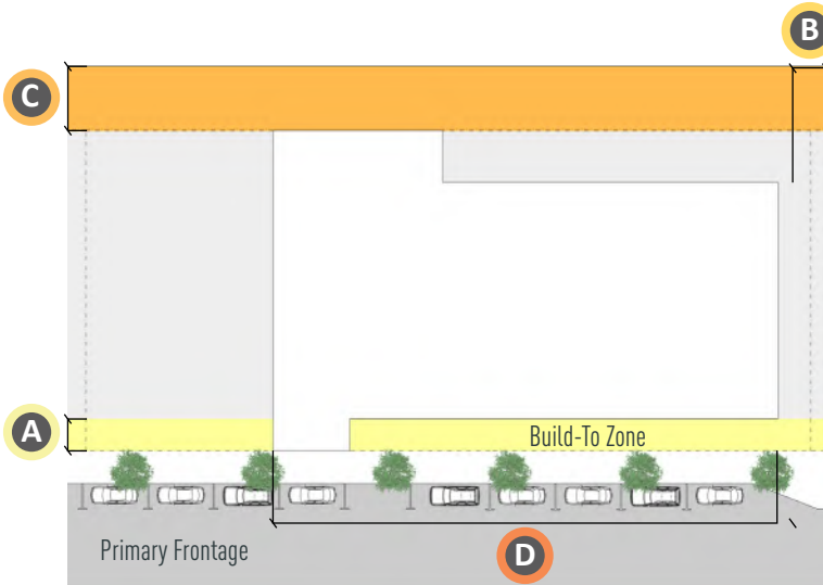
Figure 3.8 | Non-Residential Setbacks
